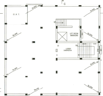
BLOCK - A ROOF PLAN
