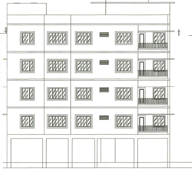
FRONT ELEVATION (BLOCK-A) SCALE: 1:100
